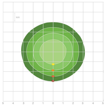
UDD 65 G3 5K MOUNTING HEIGHT: 15FT
